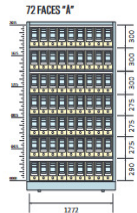
FACES | ESCALA 1:50
